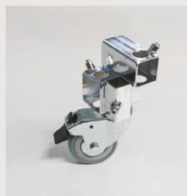
410RA3 Rollenadapter, 3-fach Caster holder, threefold for □ 20, 25, 30, 40 mm ● 16, 20, 25 mm
